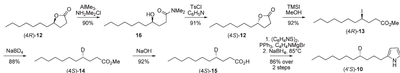
Scheme 2. Synthesis of [ 4' - ^2\text{H} ]( 4'S )-2-Undecylpyrrole [( 4'S )-10]
