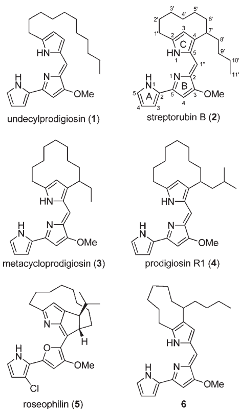
Figure 1. Structures of some of the prodiginine alkaloids 1–5 produced by actinomycetes and the incorrect structure 6 originally proposed for streptorubin B (2).
