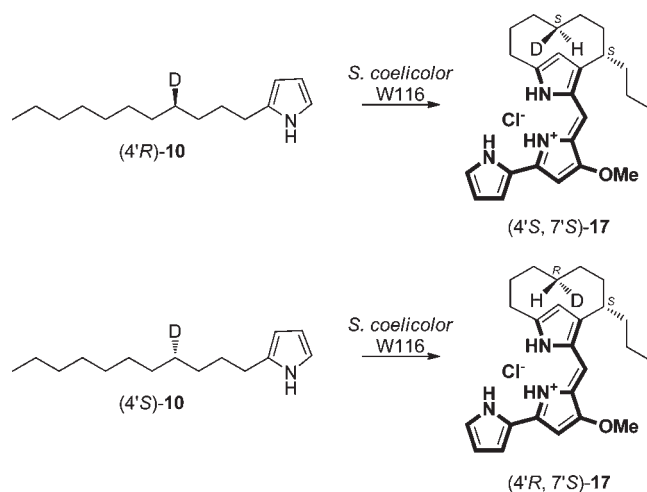
Scheme 3. Relative and Absolute Stereochemistry Assigned to the Stereoselectively Deuterium-Labeled Streptorubin B Derivatives 17 Produced by Mutasynthesis
