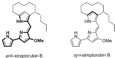
Figure 2. Structures of the anti and syn atropisomeric diastereomers of streptorubin B that arise from restricted rotation about the C-1'—C-2 C and C-7'—C-4 C bonds.
