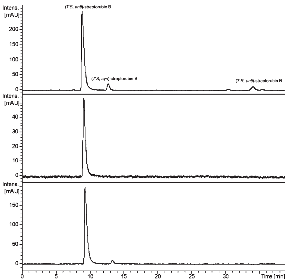
Figure 5. Chromatograms from HPLC analyses on a homochiral stationary phase of streptorubin B isolated from S. coelicolor M511 (top trace), the compound with a retention time of \sim 9.5 min analyzed immediately after collection (middle trace), and that compound analyzed after it was allowed to stand for 7 days at room temperature (bottom trace).
