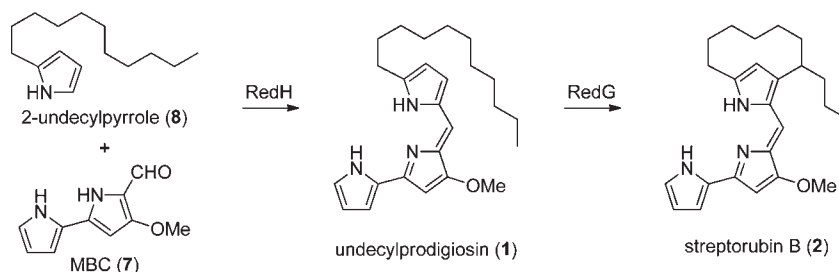
Figure 3. Pathway for the biosynthesis of undecylprodigiosin ( 1 ) and streptorubin B ( 2 ) in S. coelicolor A3(2). RedH catalyzes the condensation of 2-undecylpyrrole ( 8 ) and 4-methoxy-2,2'-bipyrrole-5-carboxaldehyde (MBC, 7 ) to form 1 , which undergoes oxidative carbocyclization catalyzed by RedG to form 2 .
