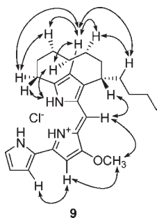
Figure 4. Key correlations observed in the NOESY NMR spectrum of streptorubin B·HCl ( 9 ) isolated from S. coelicolor M511 that establish the relative stereochemistry of the major isomer in solution.
