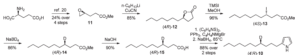
Scheme 1. Synthesis of [ 4' - ^2\text{H} ]( 4'R )-2-Undecylpyrrole [( 4'R )-10]
